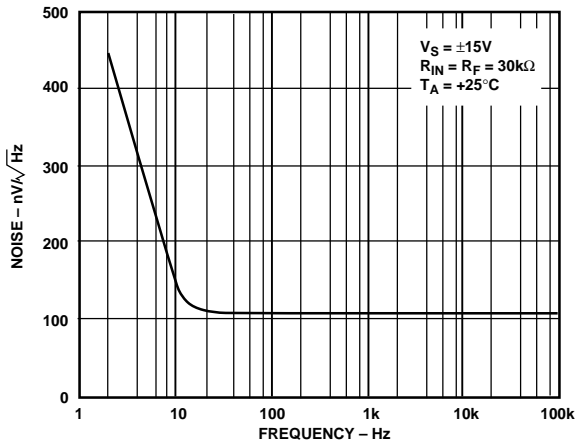
Figure 10. Voltage Noise Density vs. Frequency, Class AB
